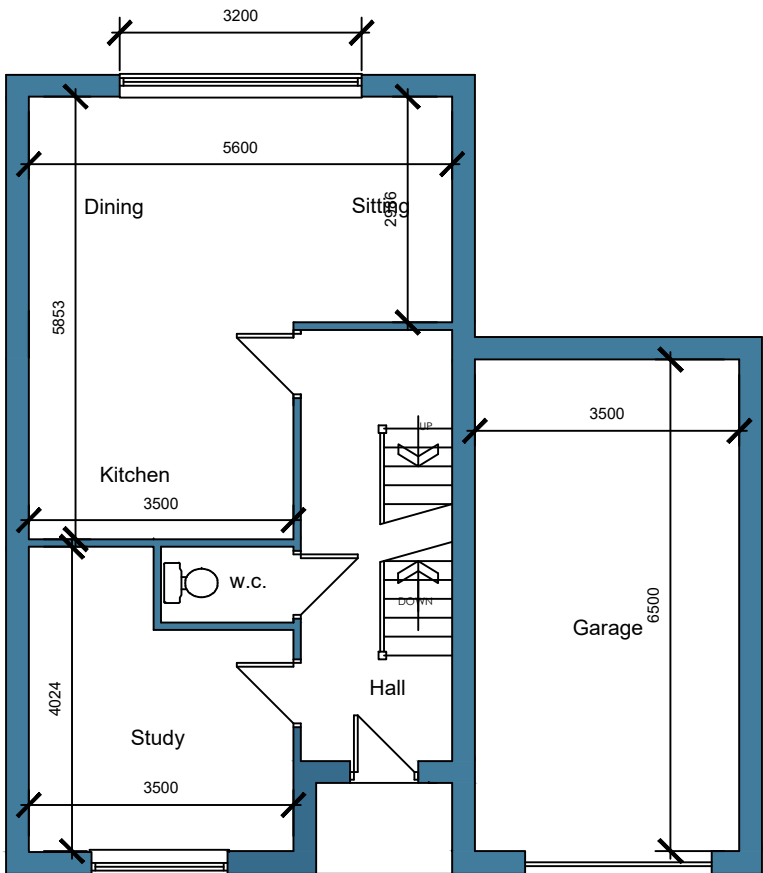
UPPER GROUND FLOOR PLAN
