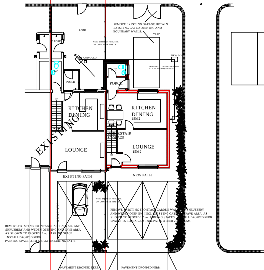
PROPOSED GROUND FLOOR PLAN AND SITE PLAN - NEW HOUSE
