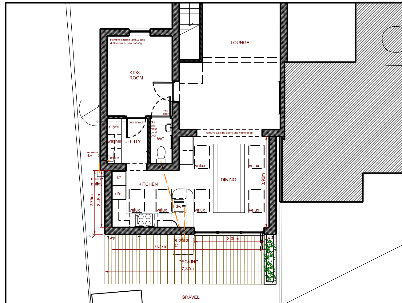
Ground Floor Plan - Proposed
