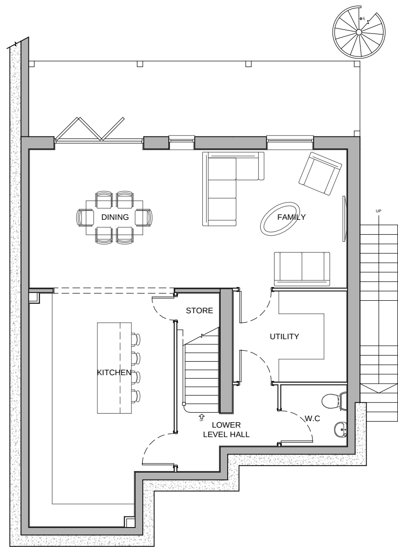
LOWER GROUND FLOOR PLAN
