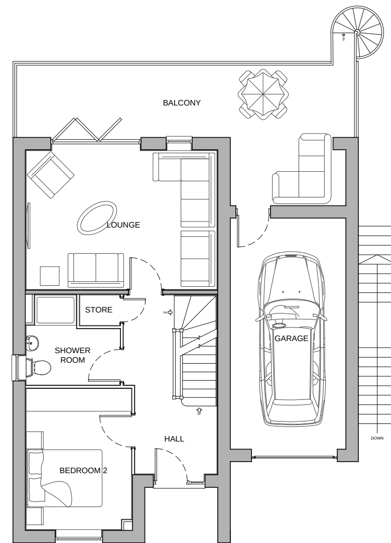
UPPER GROUND FLOOR PLAN
