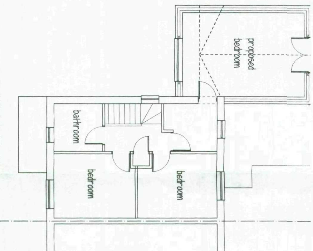
FIRST FLOOR
