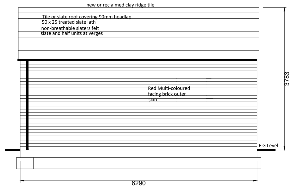
West Elevation
