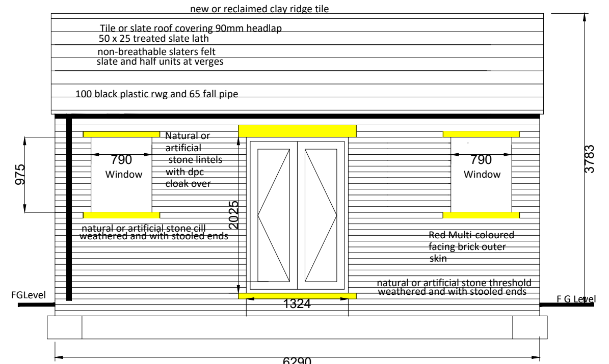
East Elevation
