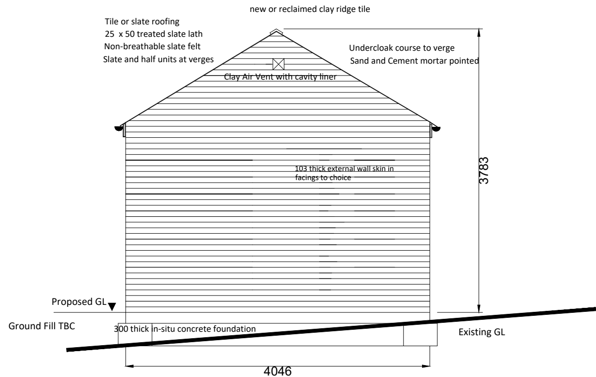
North Elevation
