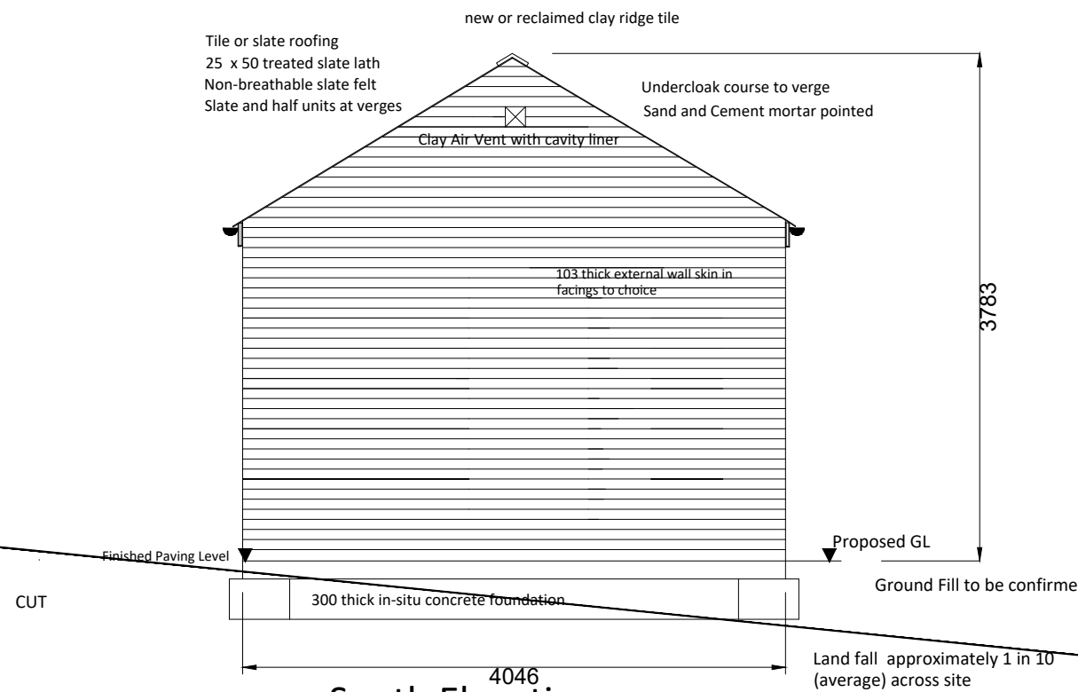
South Elevation
