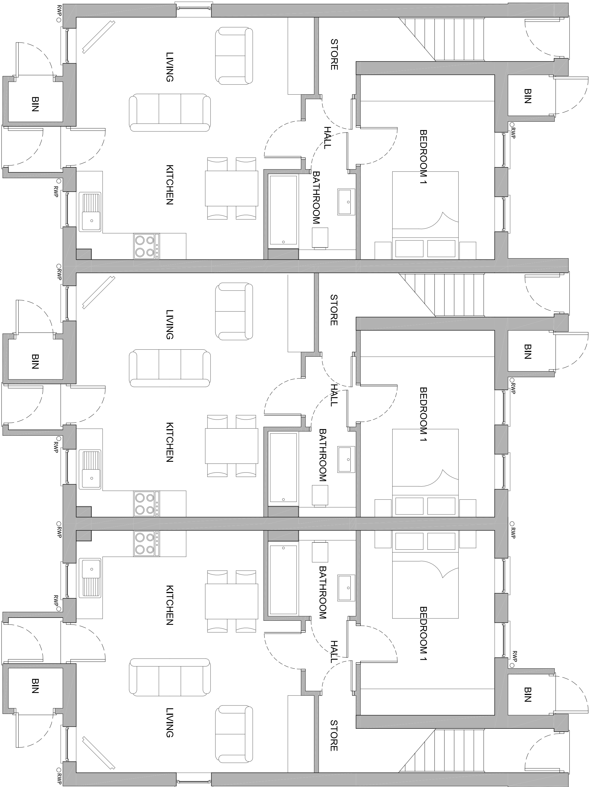
GROUND FLOOR
