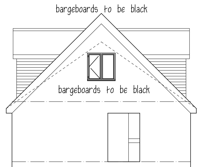
REAR ELEVATION
