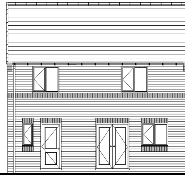
REAR ELEVATION
